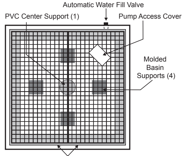
Grates (2) 48" long x 24" wide
