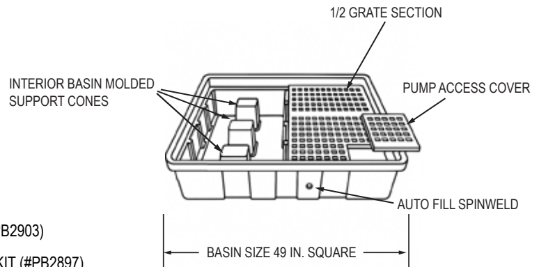
TOP VIEW BASIN/GRATE DETAIL
